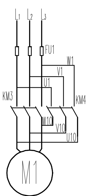
turning motor
